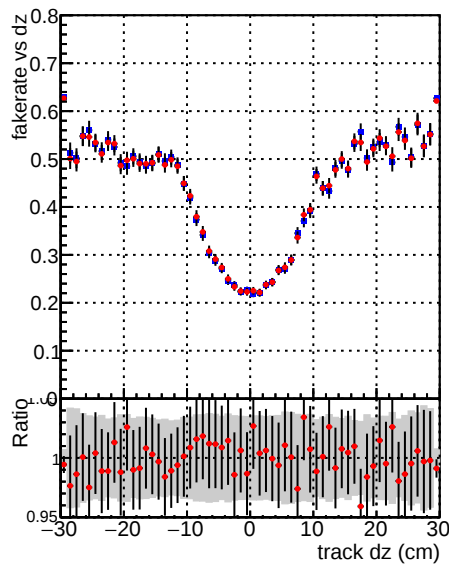
—•— DQM_mkFit_TToriginal —•— DQM_mkFit_TTNEWhoMS-genMatch-CUT
