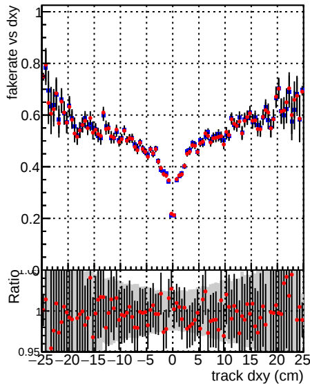
—•— DQM_mkFit_TToriginal —•— DQM_mkFit_TTNEWhoMS-genMatch-CUT
