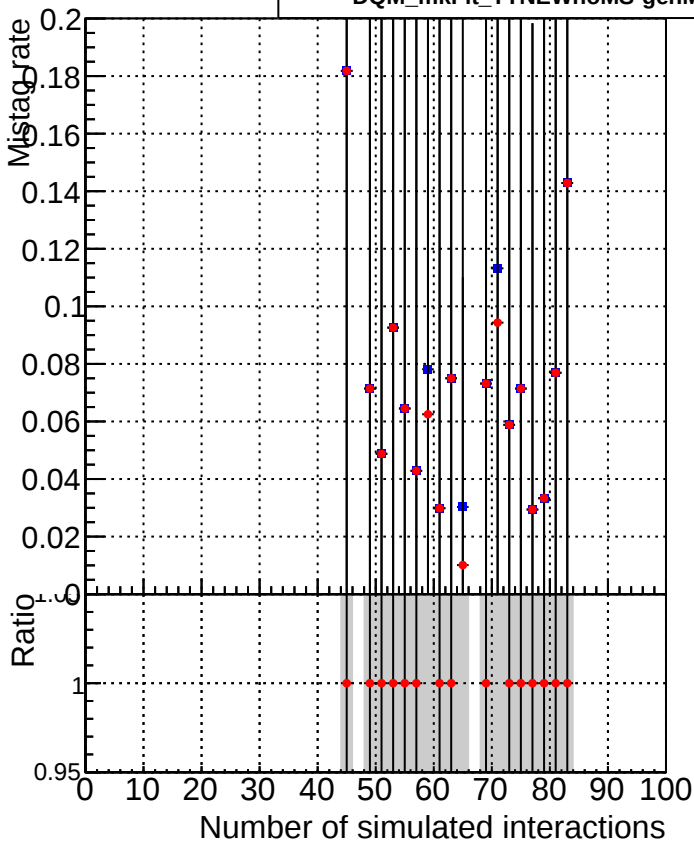
■ DQM_mkFit_TToriginal ● DQM_mkFit_TTNEWnoMS-genMatch-CUT
