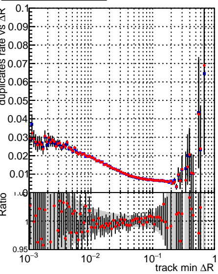
—•— DQM_mkFit_TToriginal —•— DQM_mkFit_TTNEwoMS-genMatch-CUT
