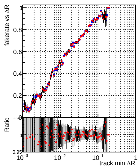
Fake rate vs \Delta R(\text{track, jet}) Legend: DQM_mkFit_TToriginal (blue line with error bars), DQM_mkFit_TTNEWnoMS-genMatch-CUT (red line with error bars)
