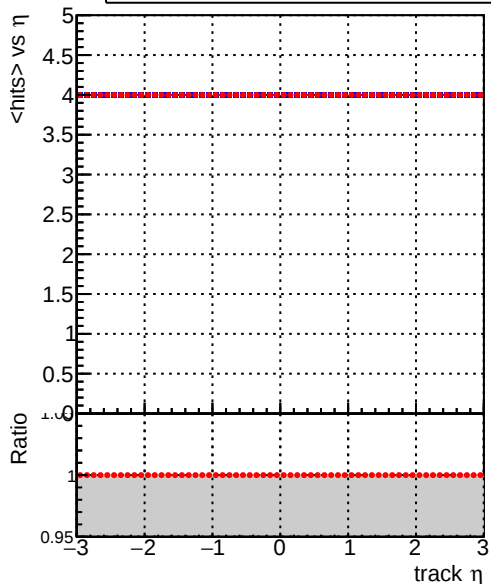
mean hit — DQM_mkFit_TToriginal — DQM_mkFit_TTNEwMS-genMatch-CUT
