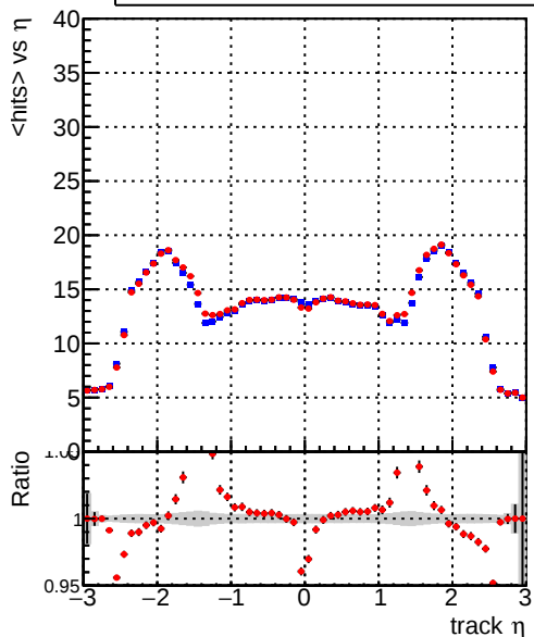
mean hits — DQM_mkFit_TToriginal — DQM_mkFit_TTNEwMS-genMatch-CUT
