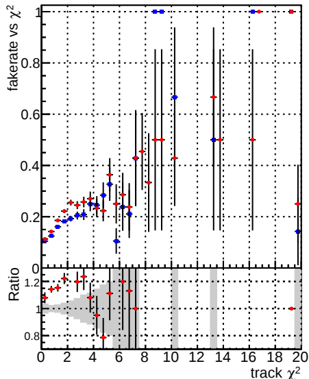
Fake rate vs. —•— DQM_mkFit_TToriginal —•— DQM_mkFit_TTNEWhoMS-genMatch-CUT
