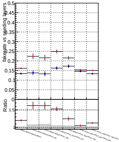
Fake rate vs. —•— DQM_mkFit_TToriginal —•— DQM_mkFit_TTNEWhoMS-genMatch-CUT
