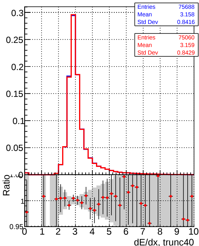
■ DQM_mkFit_TToriginal ● DQM_mkFit_TTNEWnoMS-genMatch-CUT
