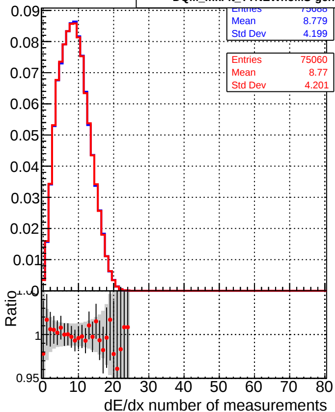
■ DQM_mkFit_TToriginal ● DQM_mkFit_TTNEWnoMS-genMatch-CUT
