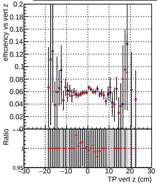
Efficiency vs. TP vert z (cm) Legend: - DQM_mkFit_TToriginal (blue line with markers) - DQM_mkFit_TTNEwMS-genMatch-CUT (red line with markers)
