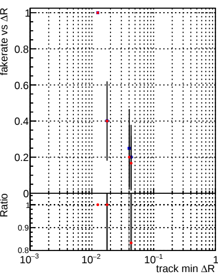
Fake rate vs \Delta R(\text{track, jet}) DQM_mkFit_TToriginal DQM_mkFit_TTNEWnoMS-genMatch-CUT
