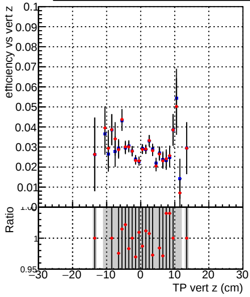
Efficiency vs vert z — DQM_mkFit_TToriginal — DQM_mkFit_TTNEwMS-genMatch-CUT
