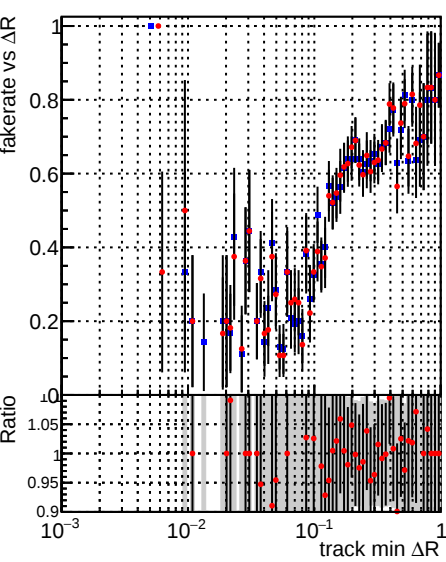
Legend: DQM_mkFit_TToriginal (blue), DQM_mkFit_TTNEwnoMS-genMatch-CUT (red)
