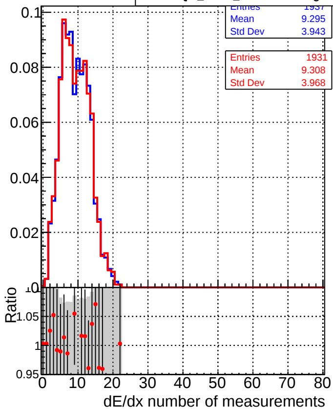
DQM_mkFit_TToriginal DQM_mkFit_TTNEwMS-genMatch-CUT
