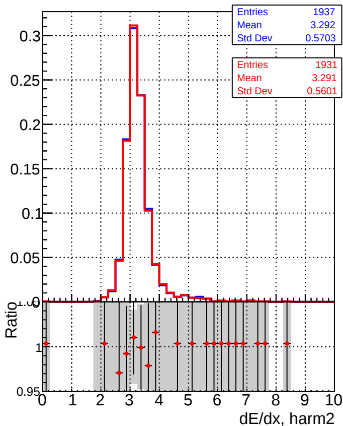
DQM_mkFit_TToriginal DQM_mkFit_TTNEwMS-genMatch-CUT
