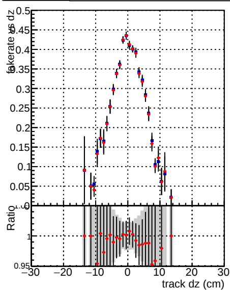
—●— DQM_mkFit_TToriginal —●— DQM_mkFit_TTNEWhoMS-genMatch-CUT
