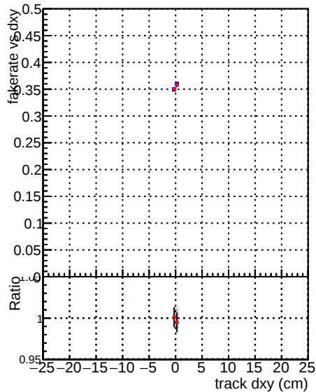
—●— DQM_mkFit_TToriginal —●— DQM_mkFit_TTNEWhoMS-genMatch-CUT
