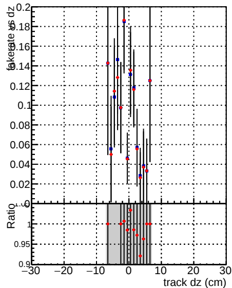
Fake rate vs dz —•— DQM_mkFit_TToriginal —•— DQM_mkFit_TTNEWhoMS-genMatch-CUT
