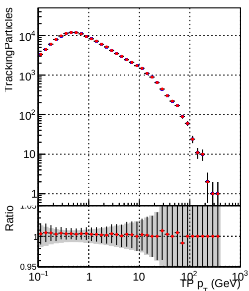
—•— DQM_mkFit_TToriginal —•— DQM_mkFit_TTNEwMS-genMatch-CUT
