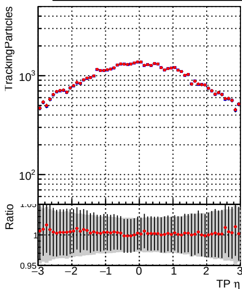
—•— DQM_mkFit_TToriginal —•— DQM_mkFit_TTNEwMS-genMatch-CUT
