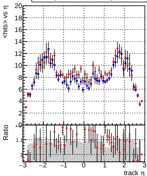
mean hits vs \eta Legend: — DQM_mkFit_TToriginal — DQM_mkFit_TTNEwMS-genMatch-CUT
