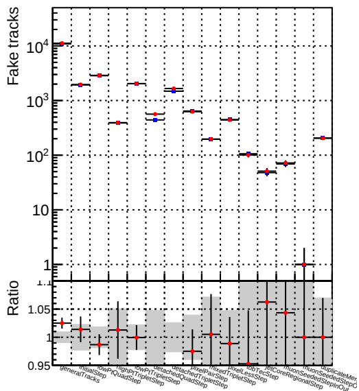
Number —●— DQM_mkFit_TTNEWnoMS-genMatch-CUT
