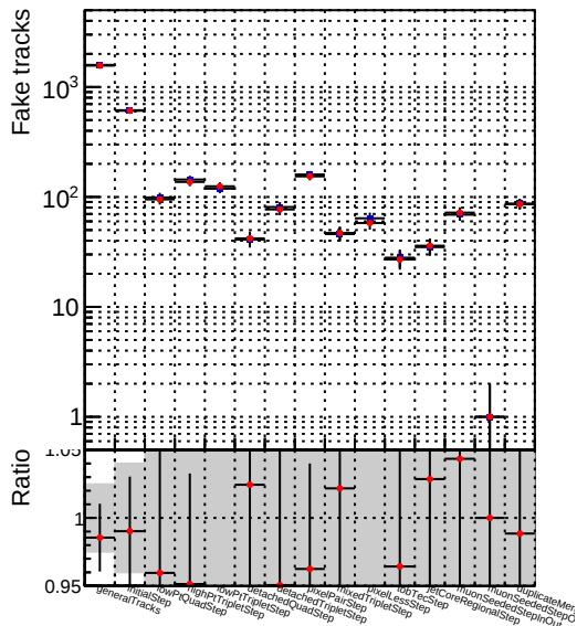
Number —●— DQM_mkFit_TTNEWnoMS-genMatch-CUT
