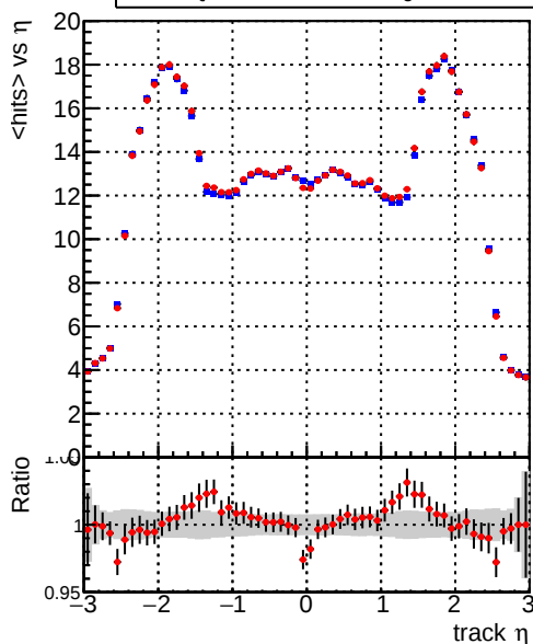
mean hit — DQM_mkFit_TToriginal — DQM_mkFit_TTNEWnoMS-genMatch-CUT
