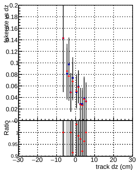
—•— DQM_mkFit_TToriginal —•— DQM_mkFit_TTNEWnoMS-genMatch-CUT
