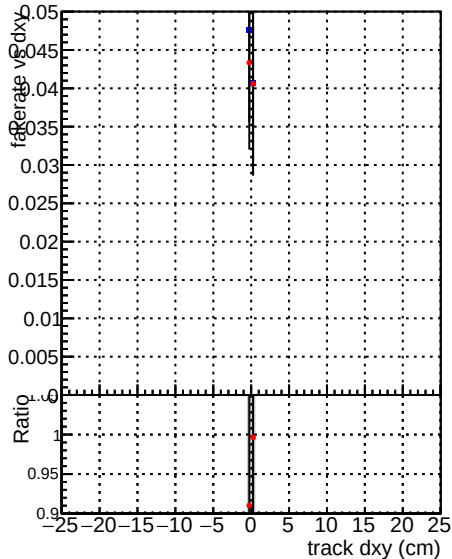
—•— DQM_mkFit_TToriginal —•— DQM_mkFit_TTNEWnoMS-genMatch-CUT
