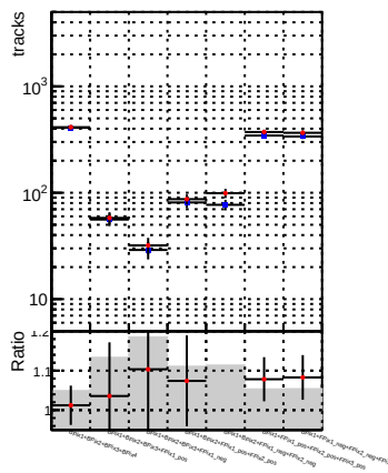
N of reco track vs. s DQM mkFit TToriginal DQM mkFit TTNEWnoMS-genMatch-CUT
