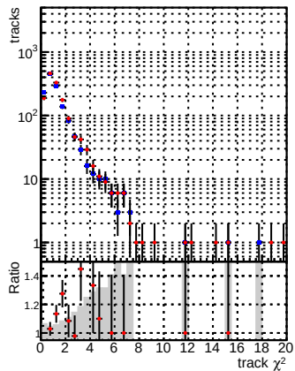
N of reco track vs. s DQM mkFit TToriginal DQM mkFit TTNEWnoMS-genMatch-CUT
