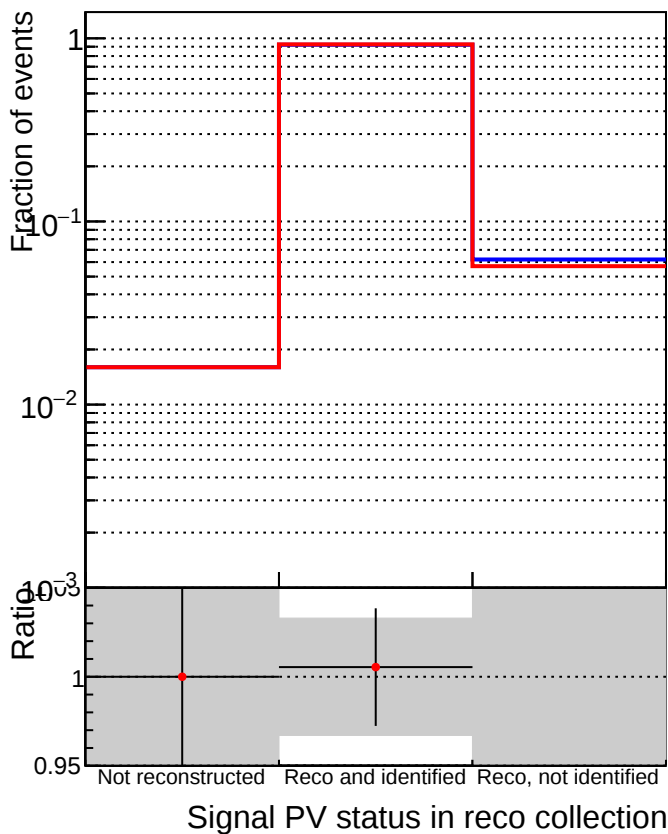
—•— DQM_mkFit_TToriginal —•— DQM_mkFit_TTNEWnoMS-genMatch-CUT
