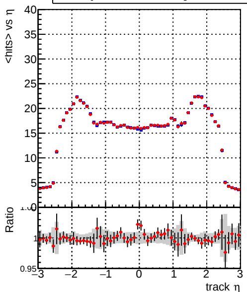
— DQM_mkFit_TToriginal — DQM_mkFit_TTNEwMS-genMatch-CUT
