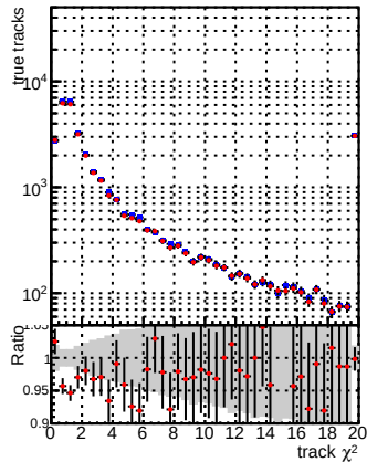
N of reco track vs. \chi^2 for DQM mkFit TToriginal and DQM mkFit TTNEWnoMS-genMatch-CUT
