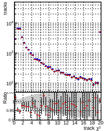
N of reco track vs. \chi^2 for DQM mkFit TToriginal and DQM mkFit TTNEWnoMS-genMatch-CUT
