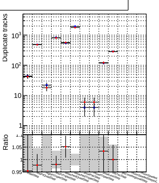
Number of duplicate tracks vs collection
