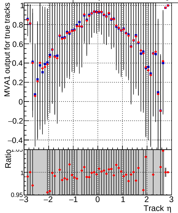
MVA1 of associated tracks (recoToSim) vs. track \eta Legend: ■ DQM_mkFit_TToriginal ● DQM_mkFit_TTNEWnoMS-genMatch-CUT
