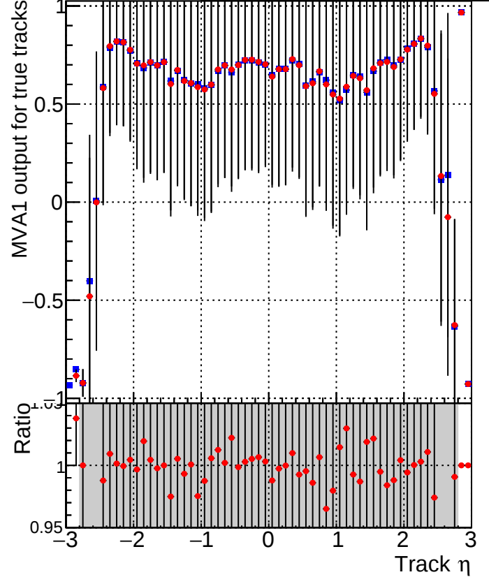
MVA1 of associated tracks (recoToSim) vs. track \eta Legend: DQM_mkFit_TToriginal (blue squares) DQM_mkFit_TTNEWnoMS-genMatch-CUT (red circles)
