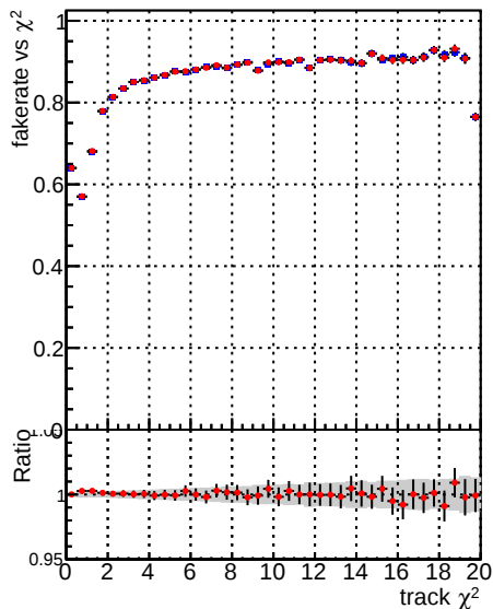
Fake rate vs. \chi^2 Legend: \square DQM_mkFit_TToriginal, \square DQM_mkFit_TTNEWhoMS-genMatch-CUT
