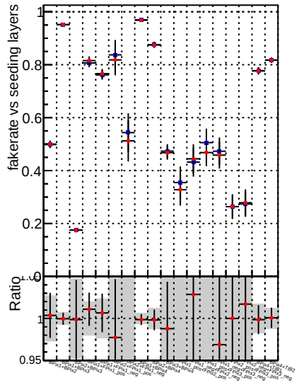
Fake rate vs. —•— DQM_mkFit_TToriginal —•— DQM_mkFit_TTNEWhoMS-genMatch-CUT
