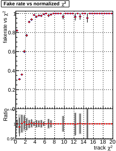
Fake rate vs. —•— DQM_mkFit_TToriginal —•— DQM_mkFit_TTNEWhoMS-genMatch-CUT
