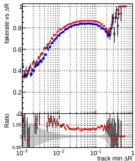
Fake rate vs DQM_mkFit_TToriginal DQM_mkFit_TTNEwMS-genMatch-CUT
