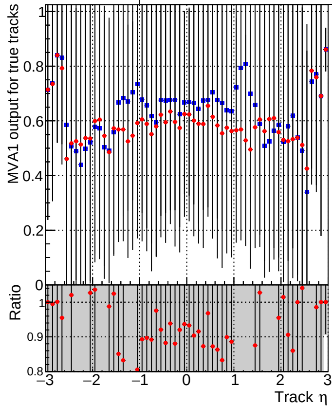
MVA1 of associated tracks (recoToSim) vs. track \eta Legend: DQM_mkFit_TToriginal (blue squares) DQM_mkFit_TTNEWnoMS-genMatch-CUT (red circles)
