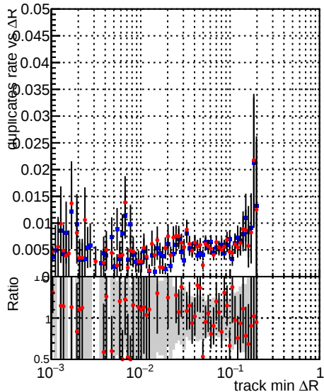
—•— DQM_mkFit_TToriginal —•— DQM_mkFit_TTNEWnoMS-genMatch-CUT
