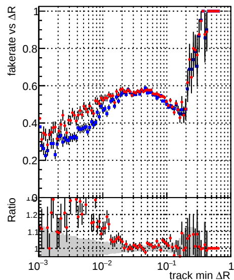
—•— DQM_mkFit_TToriginal —•— DQM_mkFit_TTNEWnoMS-genMatch-CUT
