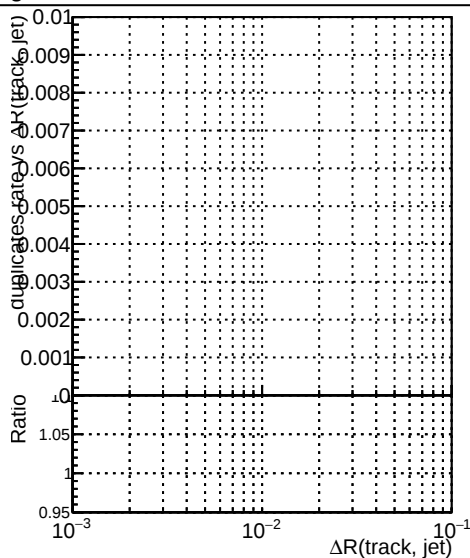
—•— DQM_mkFit_TToriginal —•— DQM_mkFit_TTNEWnoMS-genMatch-CUT
