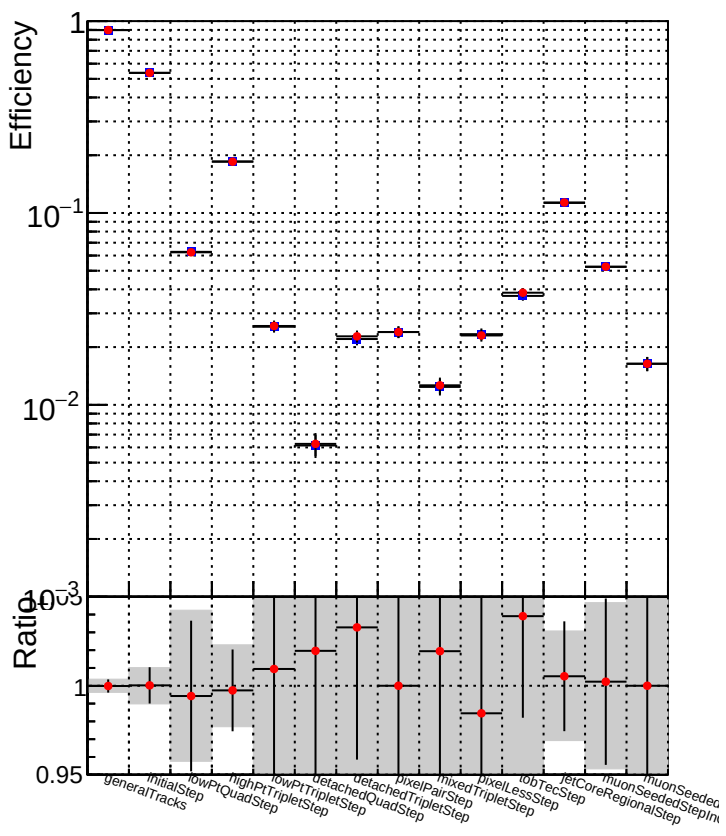
DQM_mkFit_TToriginal DQM_mkFit_TTNEWnoMS-genMatch-CUT
