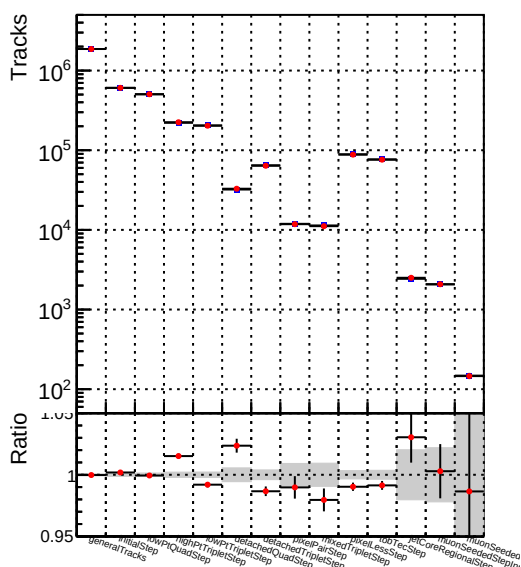
—■— DQM_mkFit_TToriginal
