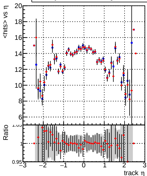
— DQM_mkFit_TToriginal — DQM_mkFit_TTNEwMS-genMatch-CUT
