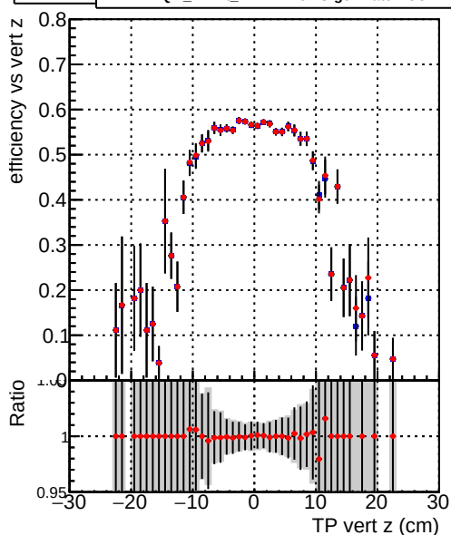
Efficiency —●— DQM_mkFit_TTNEWnoMS-genMatch-CUT
