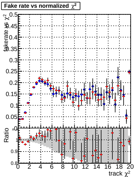
Fake rate vs. ● DQM mkFit TToriginal ★ DQM mkFit TTNEWhoMS-genMatch-CUT
