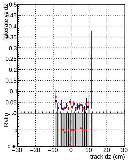
— DQM_mkFit_TToriginal — DQM_mkFit_TTNEWhoMS-genMatch-CUT
