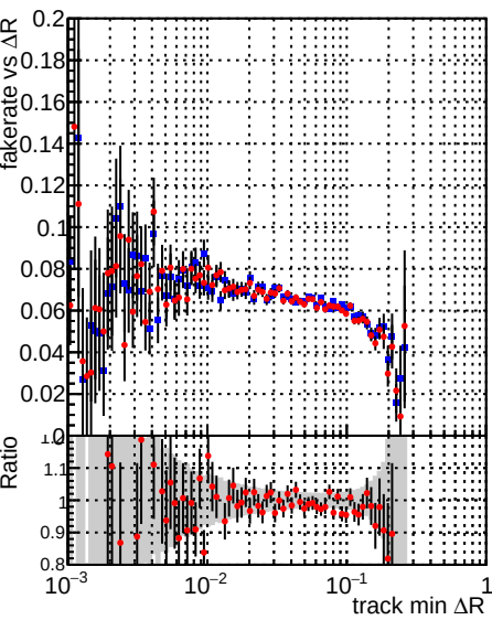
Legend: DQM_mkFit_TToriginal (blue line with error bars), DQM_mkFit_TTNEwnoMS-genMatch-CUT (red line with error bars)
