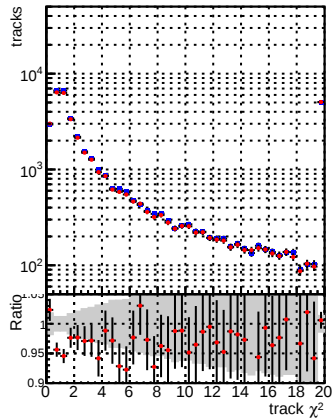
N of reco track vs. \chi^2 for DQM mkFit TToriginal (blue circles) and DQM mkFit TTNEWnoMS-genMatch-CUT (red circles).
