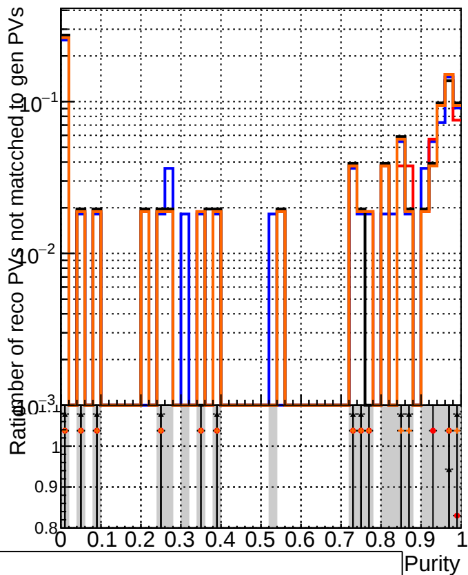
RecoPVAssoc2GenPVNotMatched_Purity
