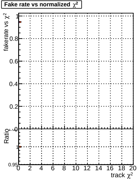
Fake rate vs. \chi^2 Legend: BGM, mkFit, TNEW, TNEW200
