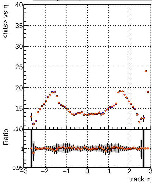
mean hits vs \eta DOM_mkFit_TToriginal DOM_mkFit_TTNEW DOM_mkFit_TTNEW50 DOM_mkFit_TTNEW100
