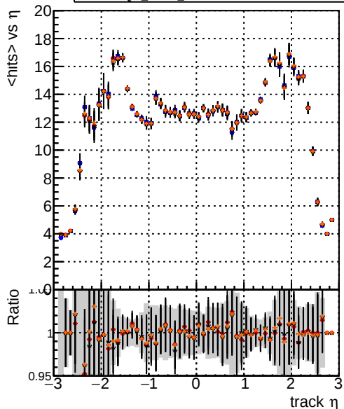
Legend: DQM_mkFit_TToriginal (blue), DQM_mkFit_TTNEW (red), DQM_mkFit_TTNEW50 (black), DQM_mkFit_TTNEW100 (orange) mean hit
