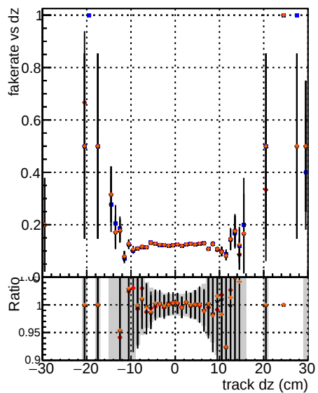
DGM mFit TNEW TNEW200 Fake rate vs d
