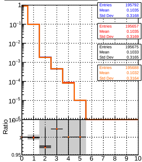
Legend: DQM_mkFit_TToriginal (blue line), DQM_mkFit_TTNEW (red line), DQM_mkFit_TTNEW50 (black line), DQM_mkFit_TTNEW100 (orange line) mean hit
