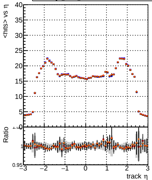
DQM_mkFit_TToriginal DQM_mkFit_TTNEW DQM_mkFit_TTNEW50 DQM_mkFit_TTNEW100 mean hits
