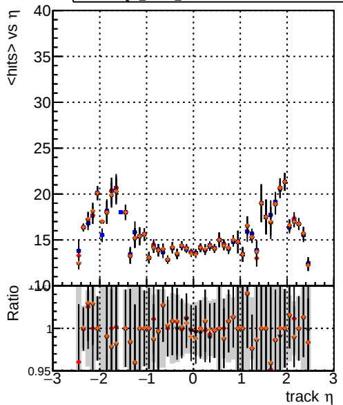
DQM_mkFit_TToriginal DQM_mkFit_TTNEW DQM_mkFit_TTNEW50 DQM_mkFit_TTNEW100 mean hit
