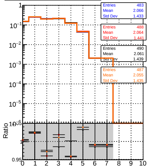
DQM_mkFit_TToriginal DQM_mkFit_TTNEW DQM_mkFit_TTNEW50 DQM_mkFit_TTNEW100
